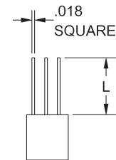
FWE WIRE WRAP 'L' 1 = .375 2 = .500 3 = .625
